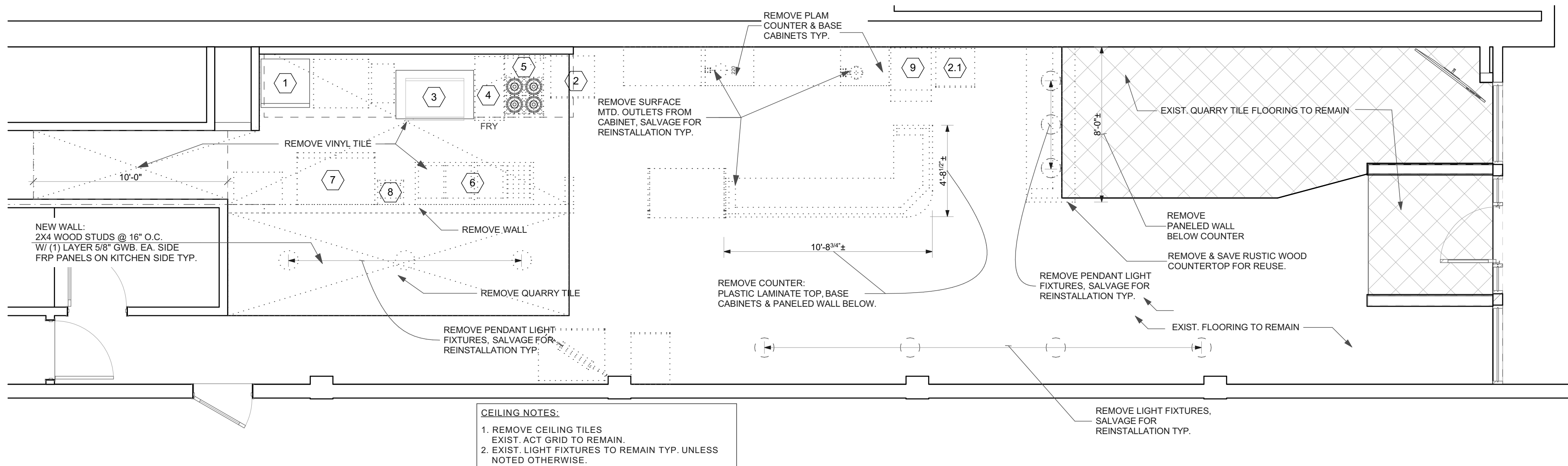
1 DEMOLITION PLAN SCALE: 1/4" = 1'-0"
