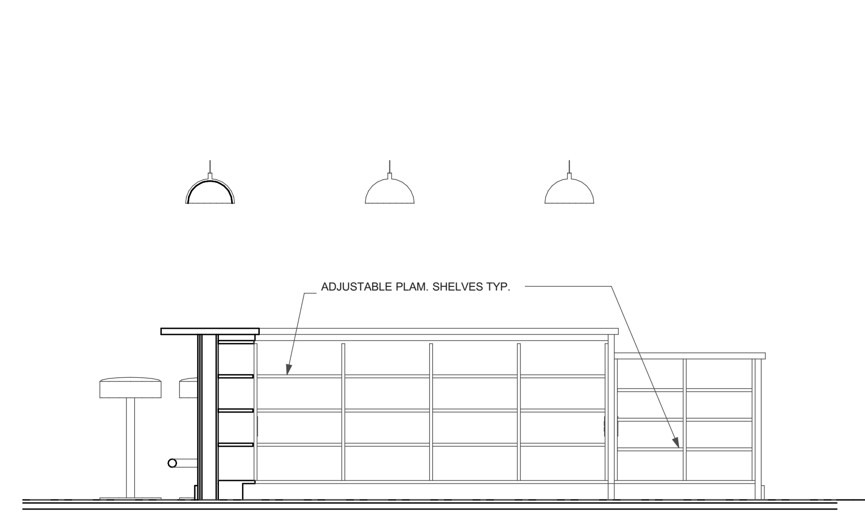
3 A-102 COUNTER SECTION/ ELEVATION SCALE: 1/2" = 1'-0"
