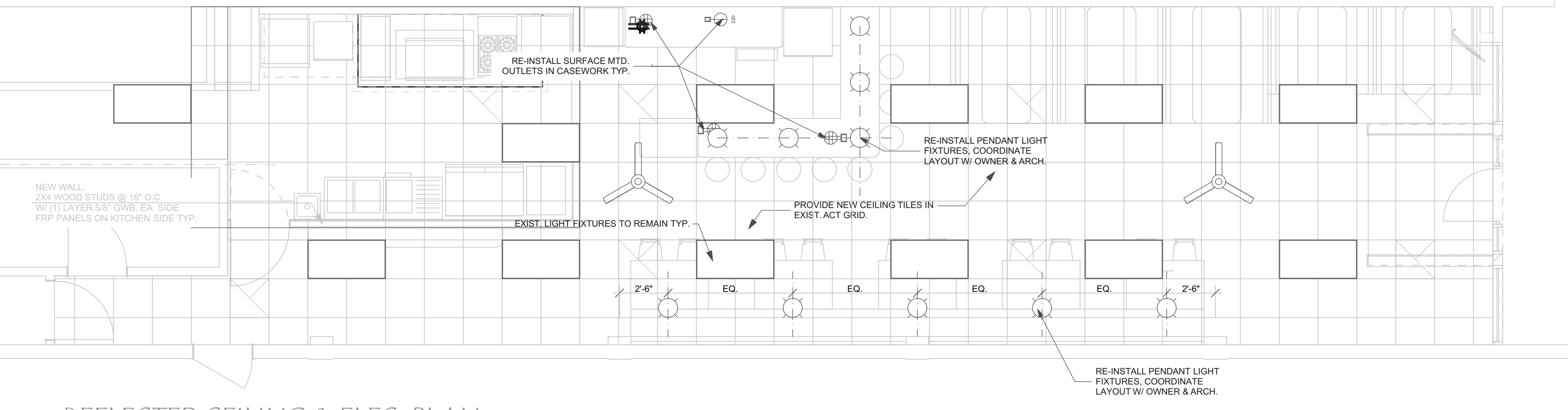
3 REFLECTED CEILING & ELEC. PLAN SCALE: 1/4" = 1'-0"
